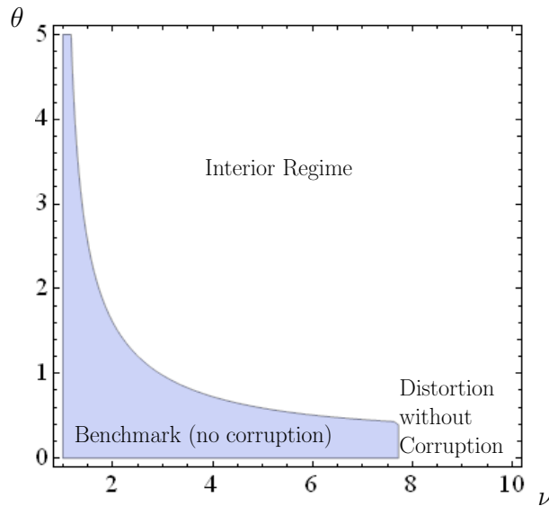
Figure 1: Regimes in the \{\nu, \theta\} plane
